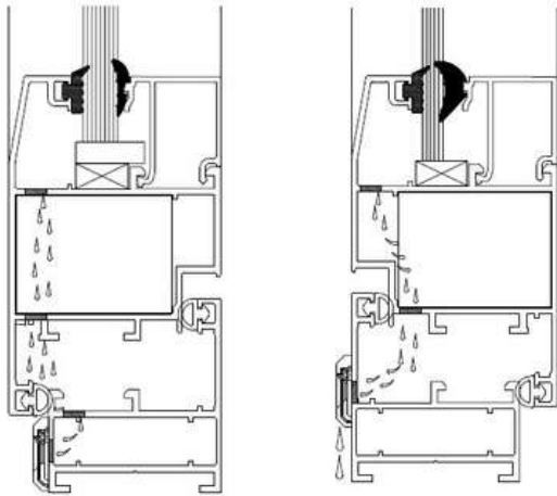
Outside Opening Window
