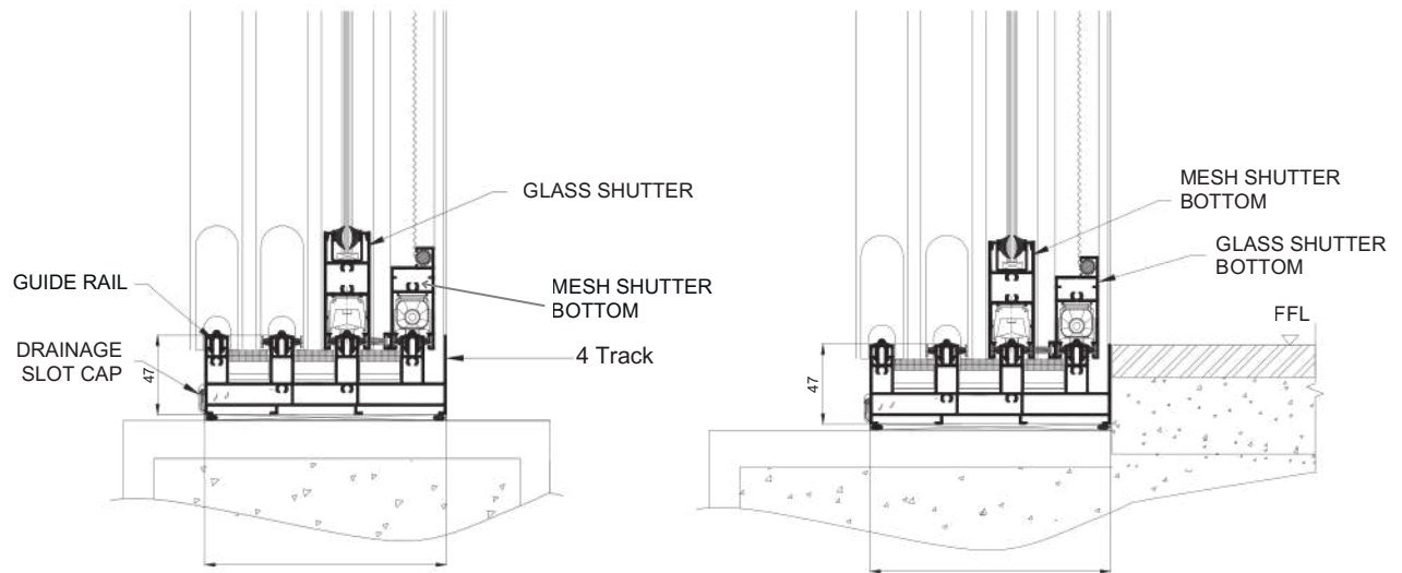
Windows on the FFL
