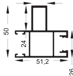
With Reinforcement
