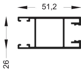
Without Reinforcement
