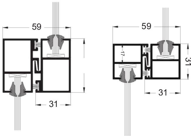
Without Reinforcement
