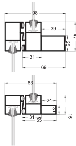
With Reinforcement
